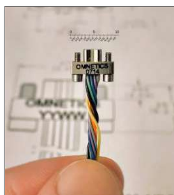
Nano D connectors 9 contacts in 4.06mm - Mil-DTL-32139 QPL Extremely rugged low profile
