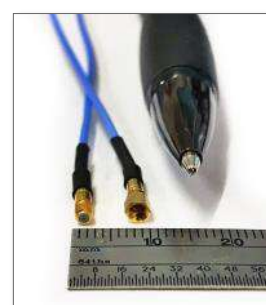
Omnetics Nano RF: 50Ω Up to 10/20 GHz
